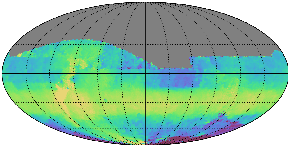
too_combined_s0.5_v3.4_10yrs All sky z band: Median HA
