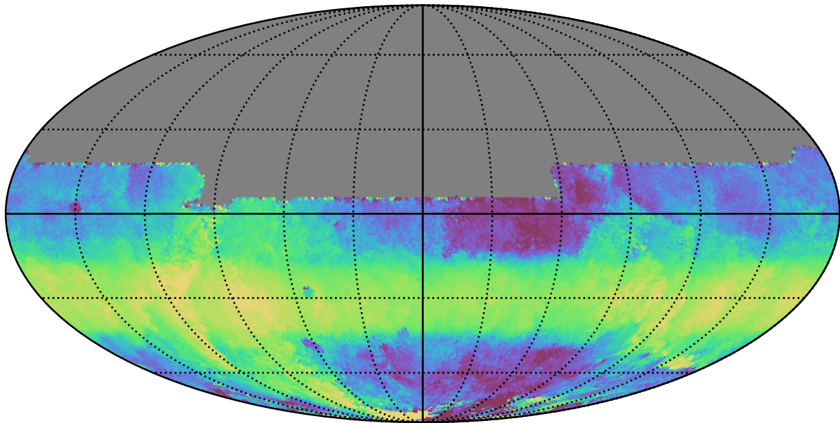
too_combined_s0.5_v3.4_10yrs All sky y band: Median HA
