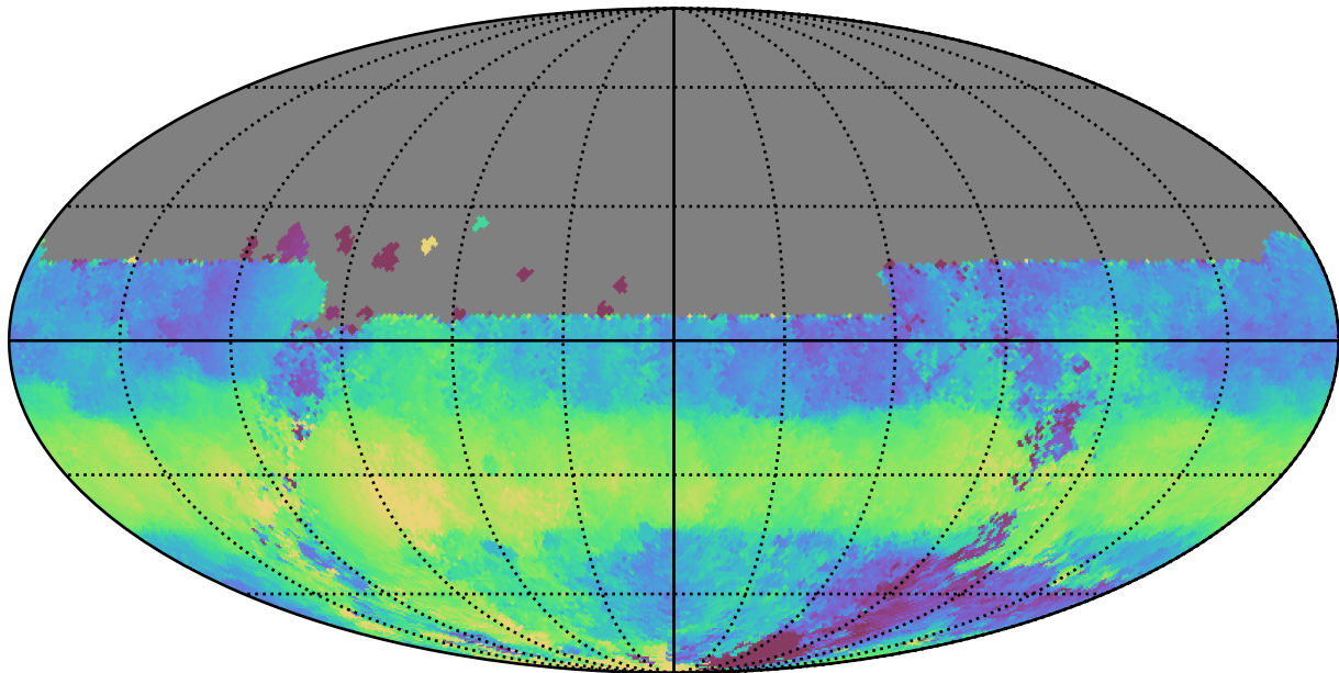
too_combined_s0.5_v3.4_10yrs All sky u band: Median HA
