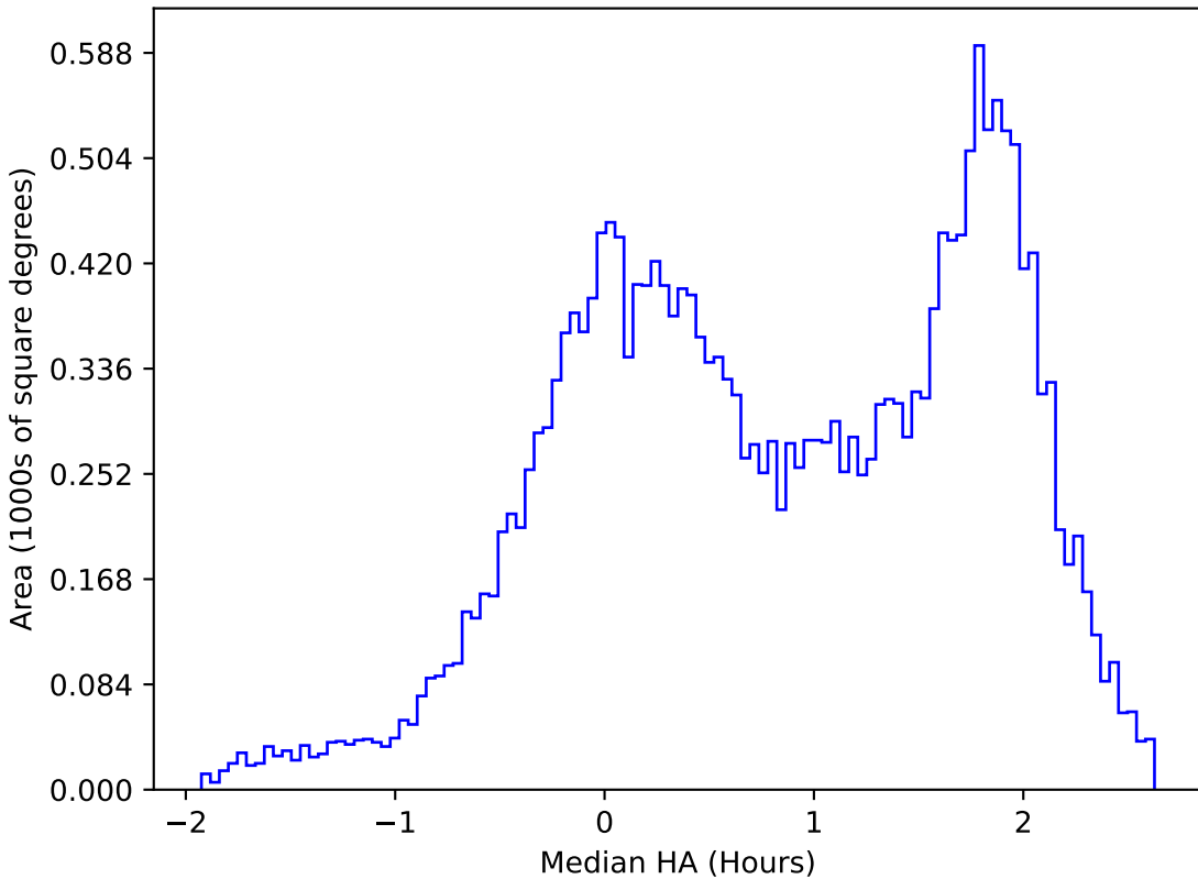
too_combined_s0.5_v3.4_10yrs All sky u band: Median HA
