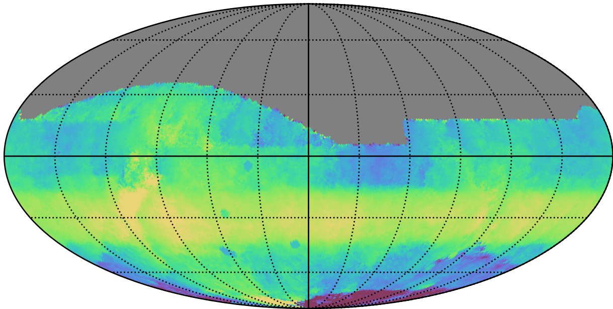
too_combined_s0.5_v3.4_10yrs All sky i band: Median HA
