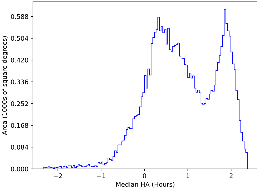
too_combined_s0.5_v3.4_10yrs All sky i band: Median HA
