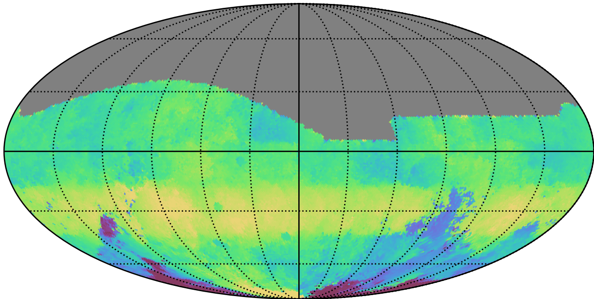
too_combined_s0.5_v3.4_10yrs All sky g band: Median HA
