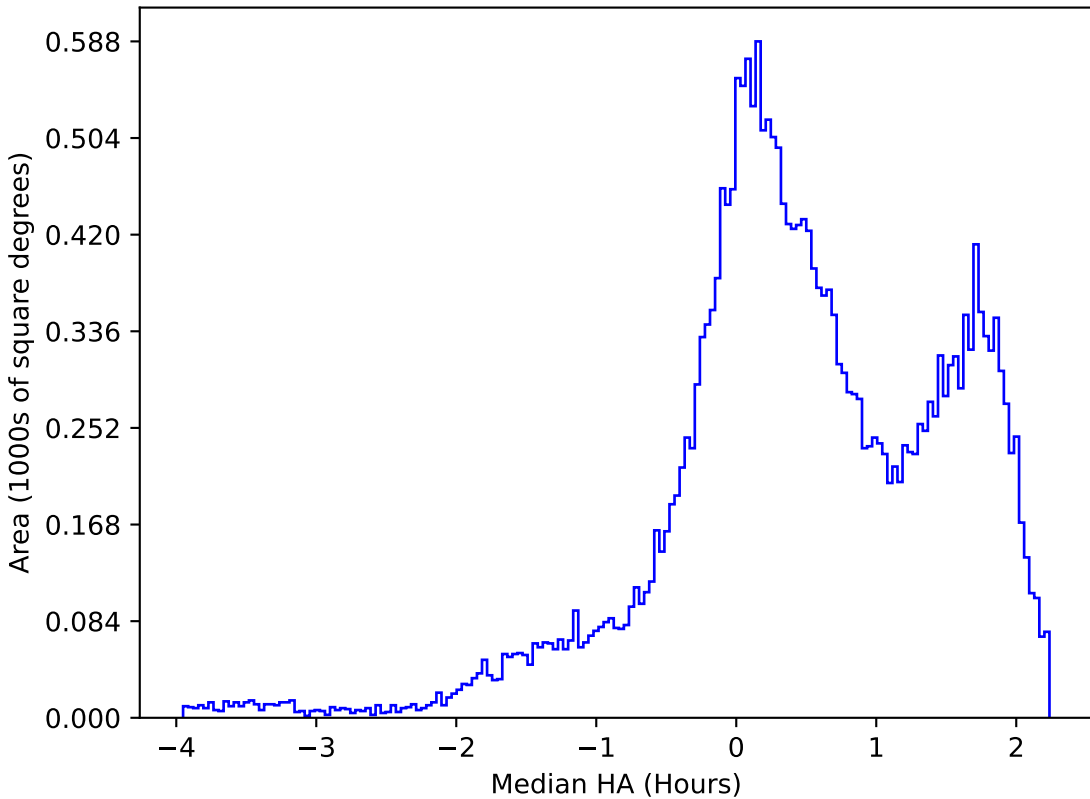
too_combined_s0.5_v3.4_10yrs All sky g band: Median HA
