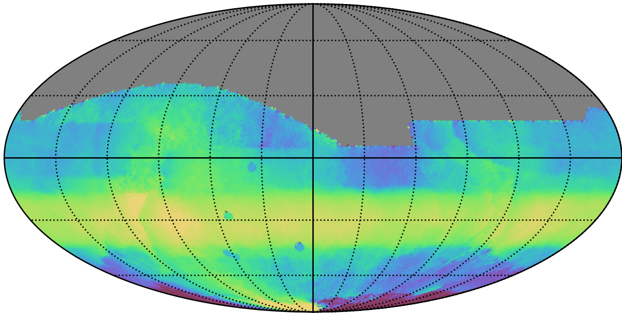
too_combined_s0.5_v3.4_10yrs All sky all bands: Median HA
