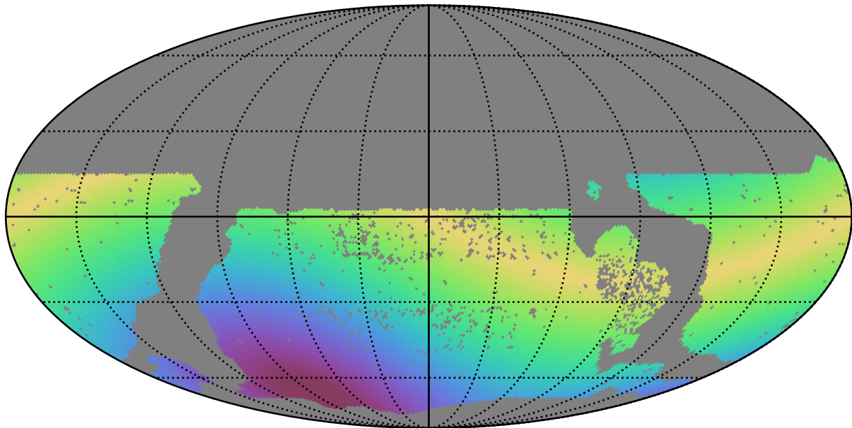
too_combined_s0.5_v3.4_10yrs WFD z band: Max solarElong
