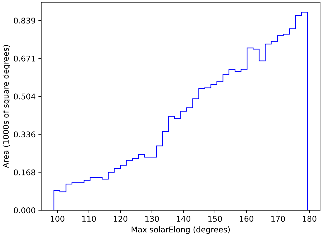
too_combined_s0.5_v3.4_10yrs WFD y band: Max solarElong
