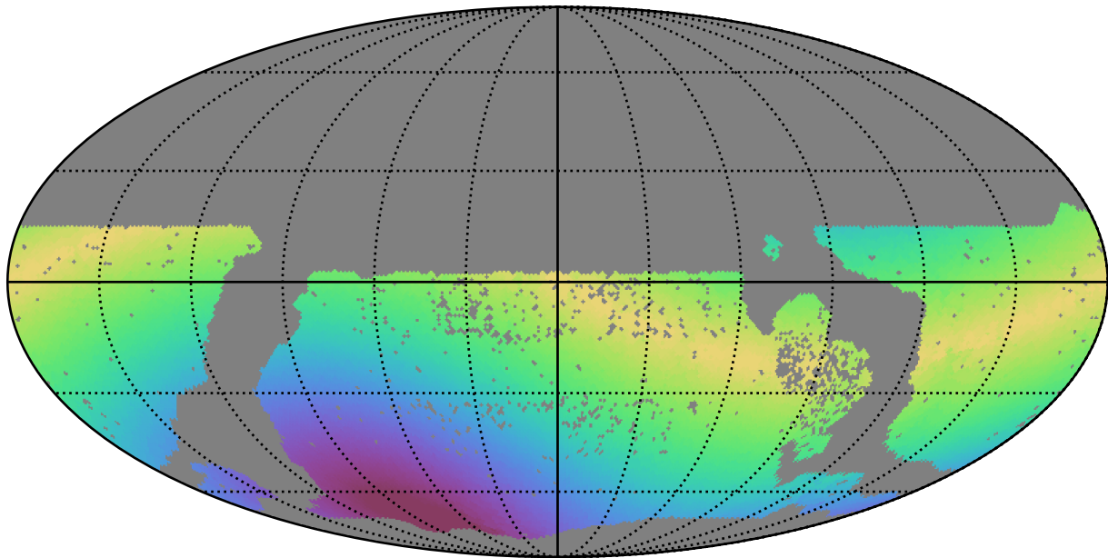
too_combined_s0.5_v3.4_10yrs WFD u band: Max solarElong
