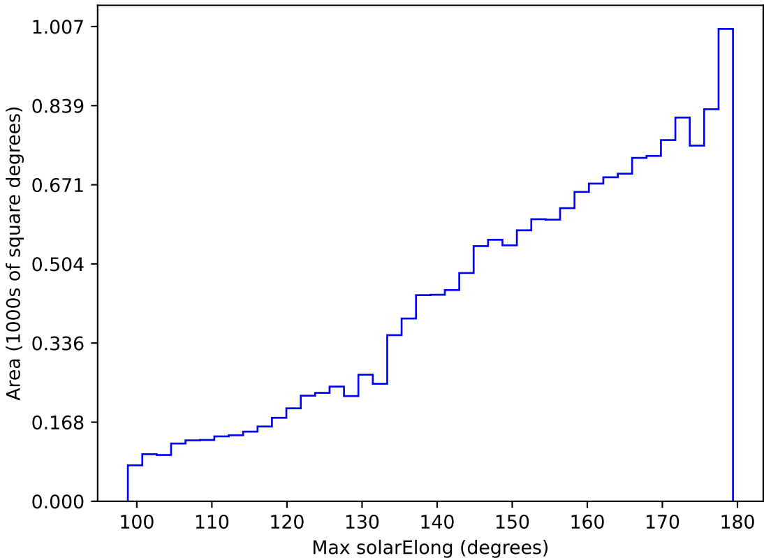
too_combined_s0.5_v3.4_10yrs WFD r band: Max solarElong
