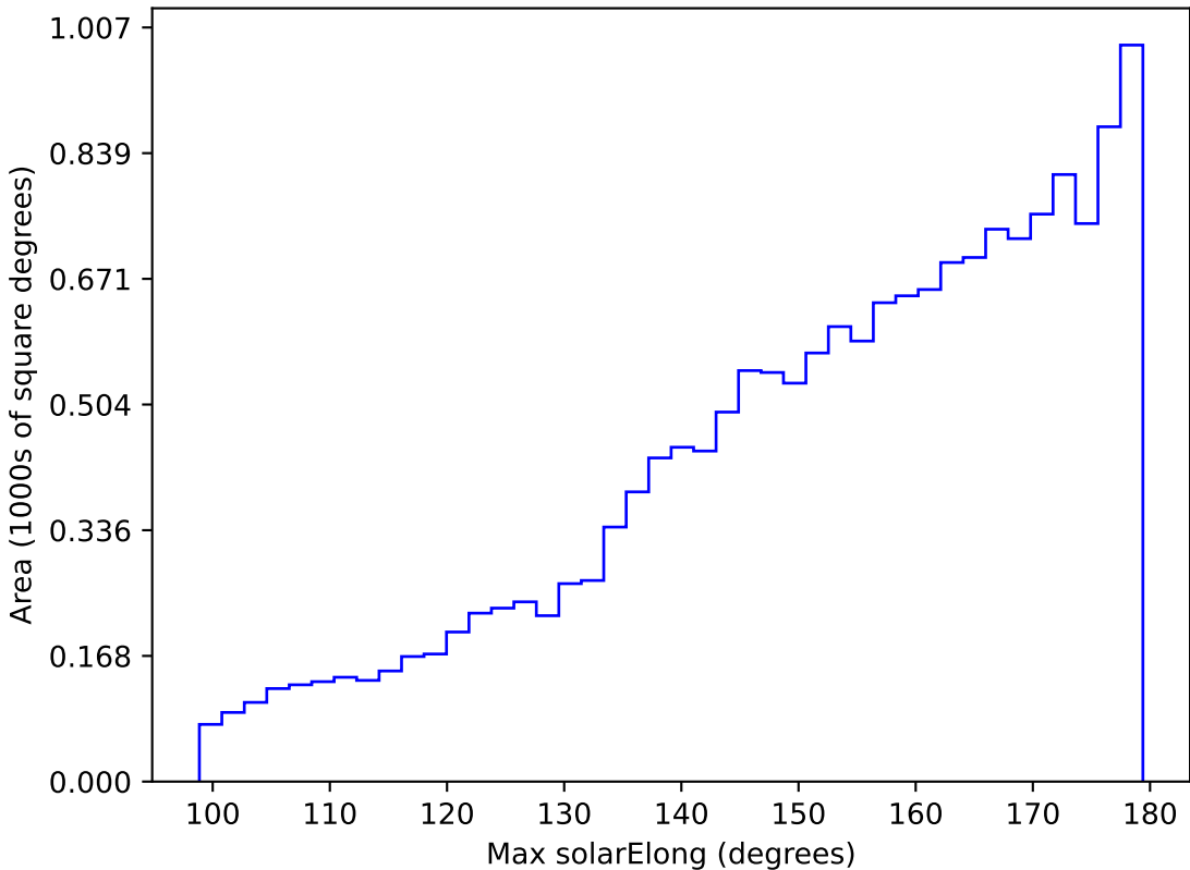
too_combined_s0.5_v3.4_10yrs WFD i band: Max solarElong
