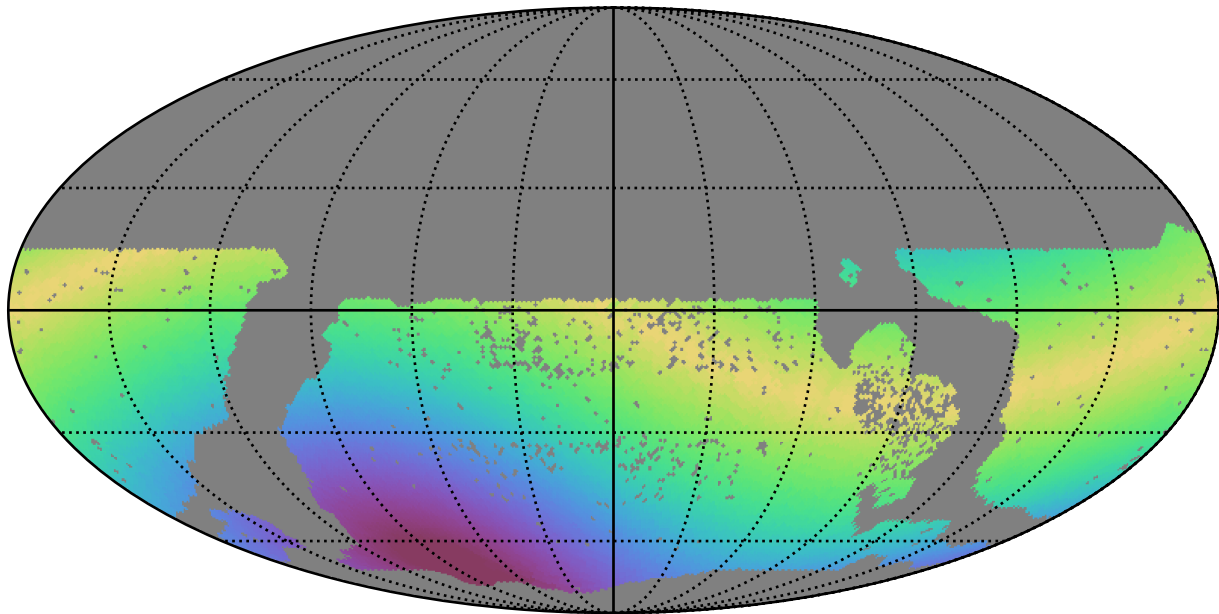
too_combined_s0.5_v3.4_10yrs WFD g band: Max solarElong
