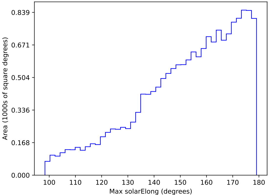
too_combined_s0.5_v3.4_10yrs WFD g band: Max solarElong
