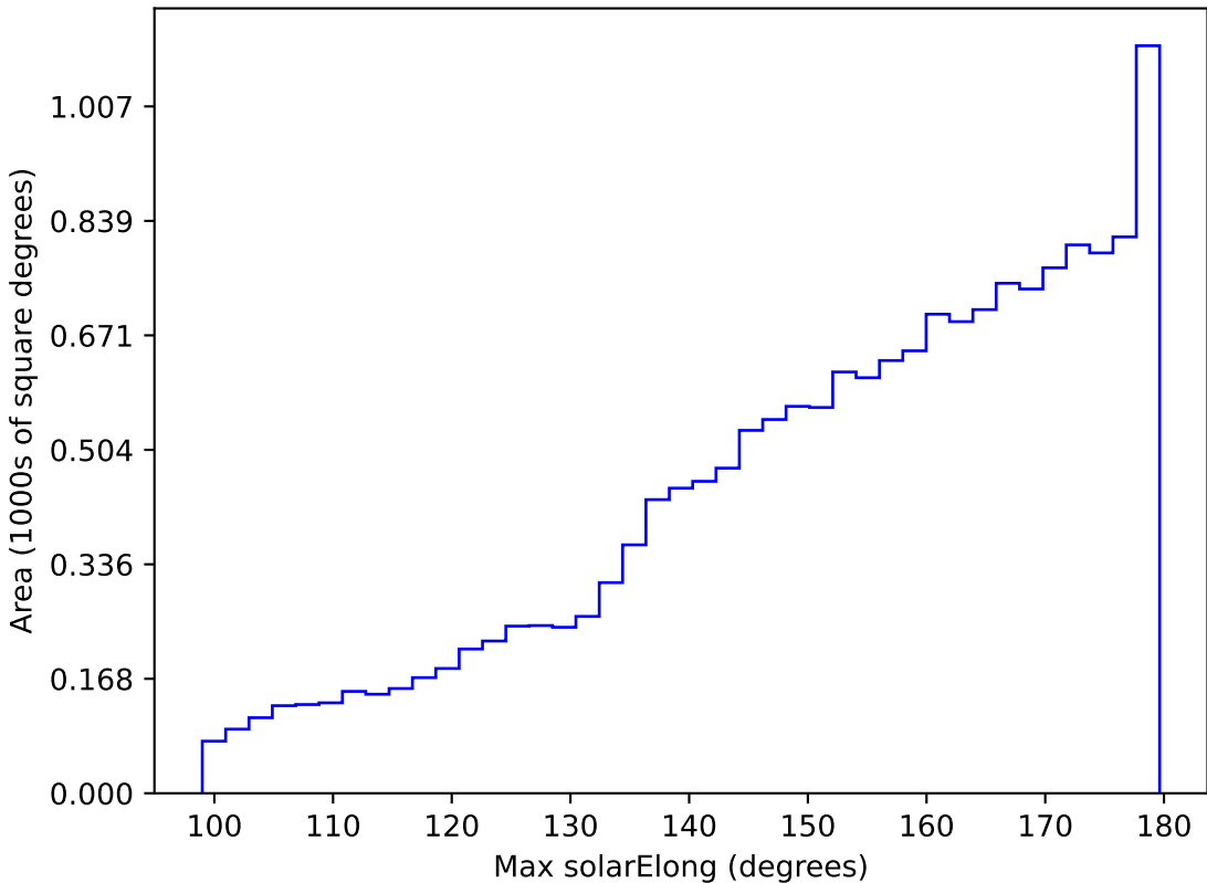
too_combined_s0.5_v3.4_10yrs WFD all bands: Max solarElong
