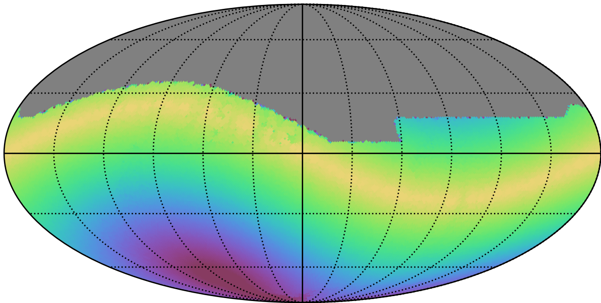
too_combined_s0.5_v3.4_10yrs All sky z band: Max solarElong
