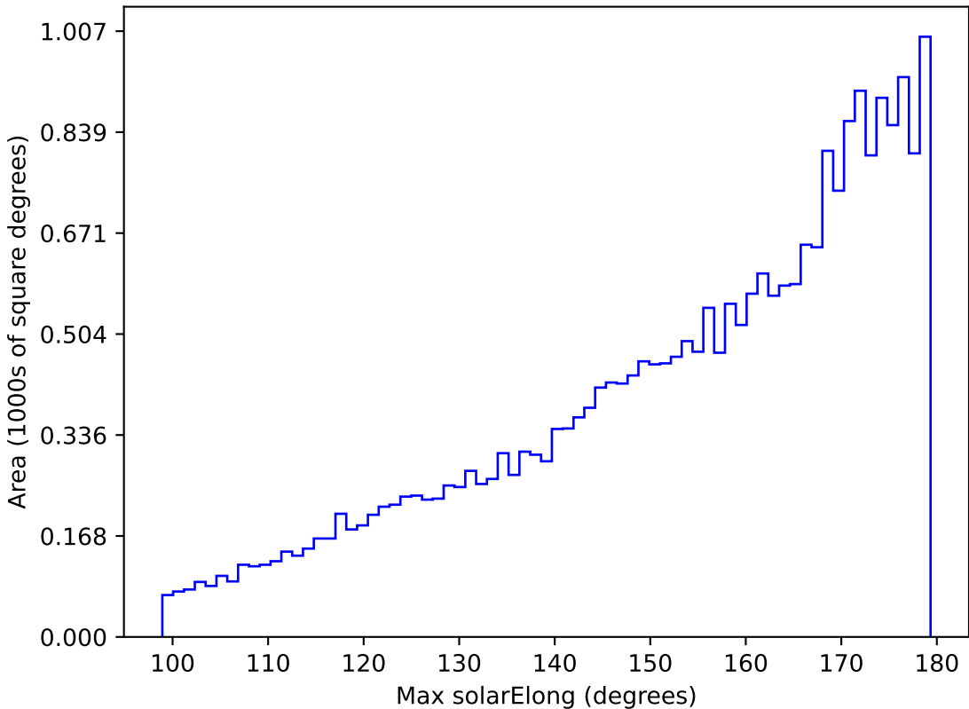
too_combined_s0.5_v3.4_10yrs All sky z band: Max solarElong
