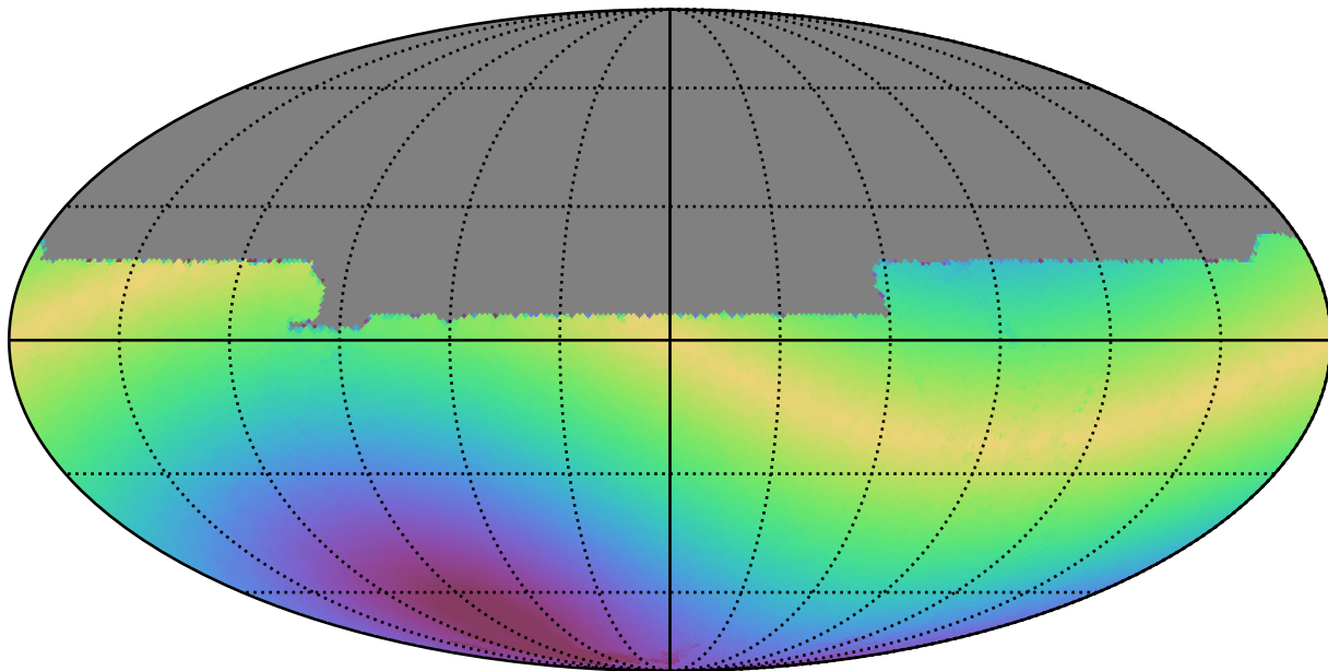
too_combined_s0.5_v3.4_10yrs All sky y band: Max solarElong
