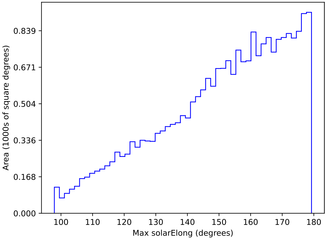
too_combined_s0.5_v3.4_10yrs All sky y band: Max solarElong
