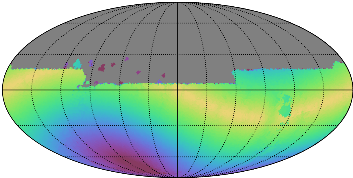
too_combined_s0.5_v3.4_10yrs All sky u band: Max solarElong
