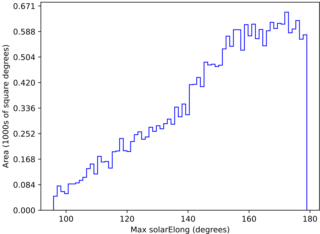
too_combined_s0.5_v3.4_10yrs All sky u band: Max solarElong
