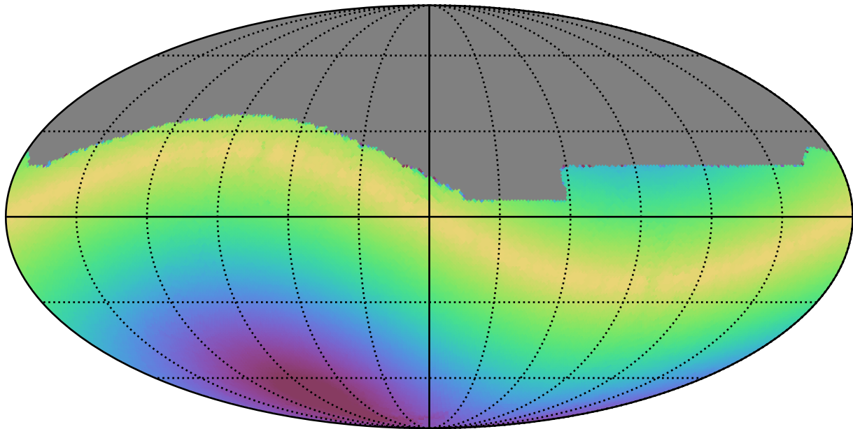
too_combined_s0.5_v3.4_10yrs All sky r band: Max solarElong
