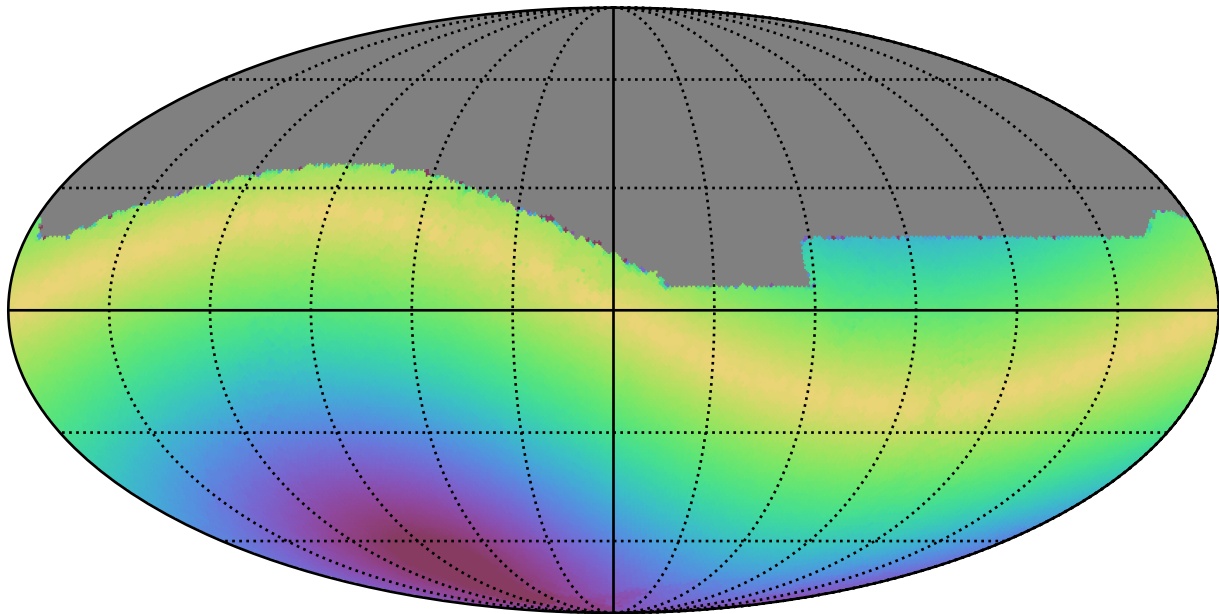
too_combined_s0.5_v3.4_10yrs All sky i band: Max solarElong
