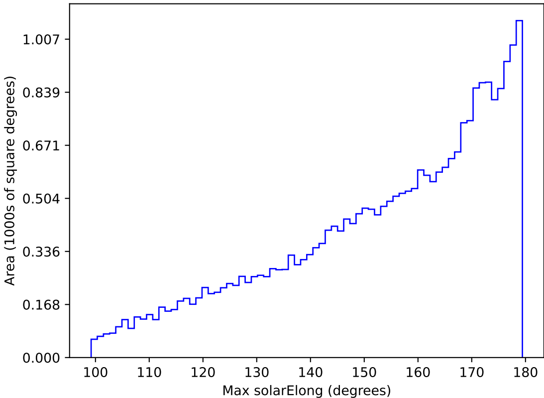
too_combined_s0.5_v3.4_10yrs All sky i band: Max solarElong
