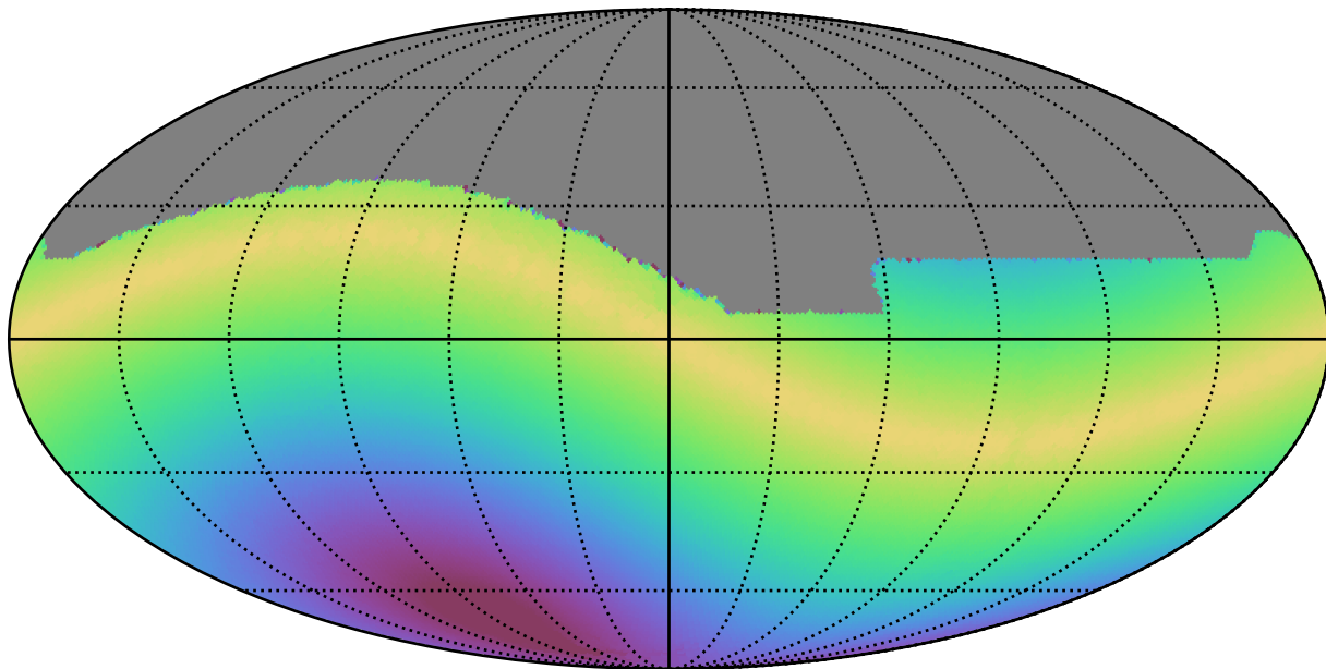
too_combined_s0.5_v3.4_10yrs All sky all bands: Max solarElong
