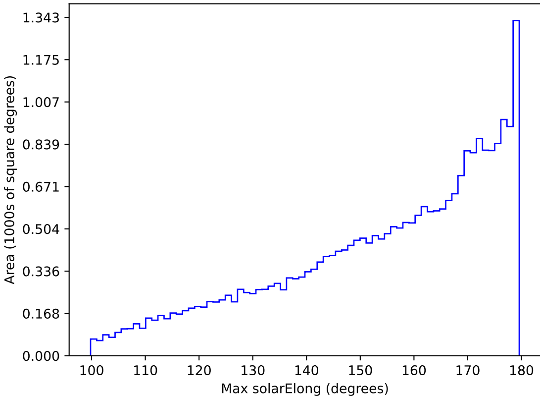
too_combined_s0.5_v3.4_10yrs All sky all bands: Max solarElong
