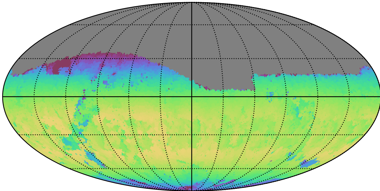
too_combined_s0.5_v3.4_10yrs Yr 1 z band: Max skyBrightness
