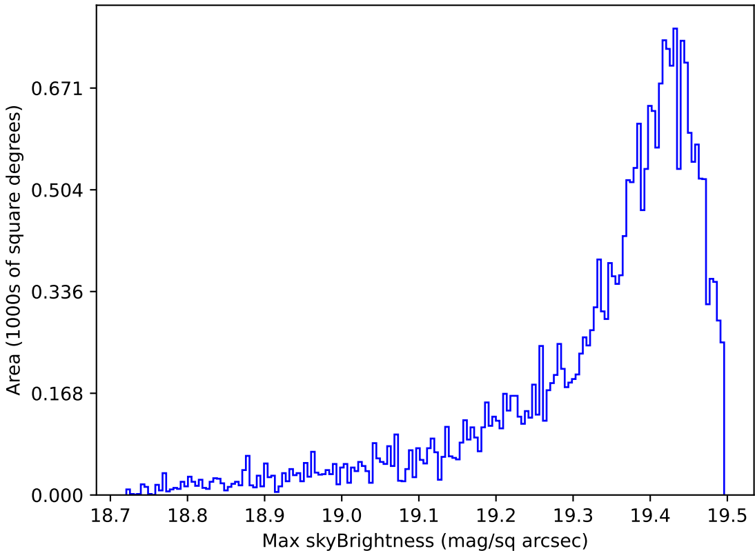
too_combined_s0.5_v3.4_10yrs Yr 1 z band: Max skyBrightness
