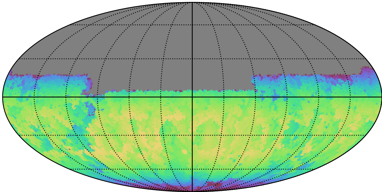
too_combined_s0.5_v3.4_10yrs Yr 1 y band: Max skyBrightness
