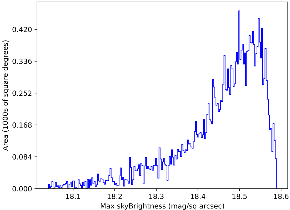
too_combined_s0.5_v3.4_10yrs Yr 1 y band: Max skyBrightness
