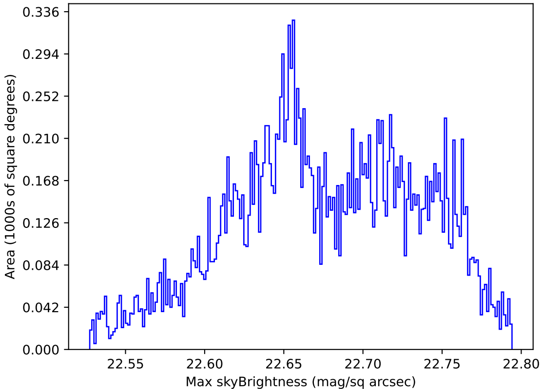
too_combined_s0.5_v3.4_10yrs Yr 1 u band: Max skyBrightness
