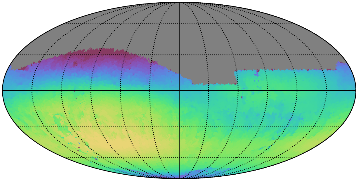
too_combined_s0.5_v3.4_10yrs Yr 1 r band: Max skyBrightness
