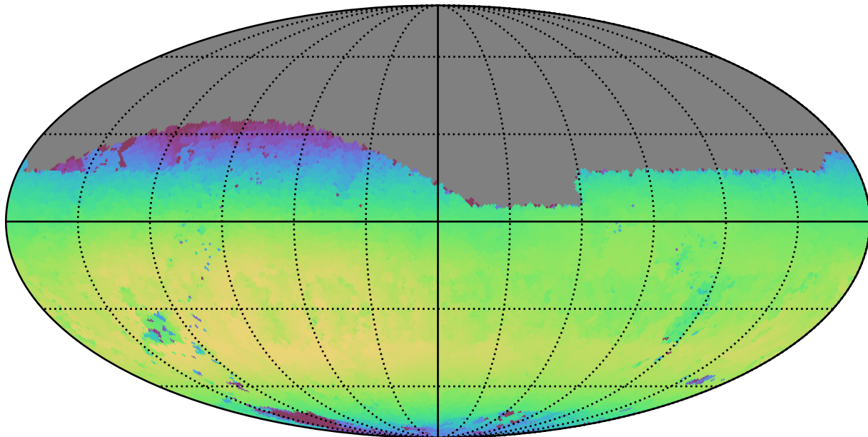
too_combined_s0.5_v3.4_10yrs Yr 1 i band: Max skyBrightness
