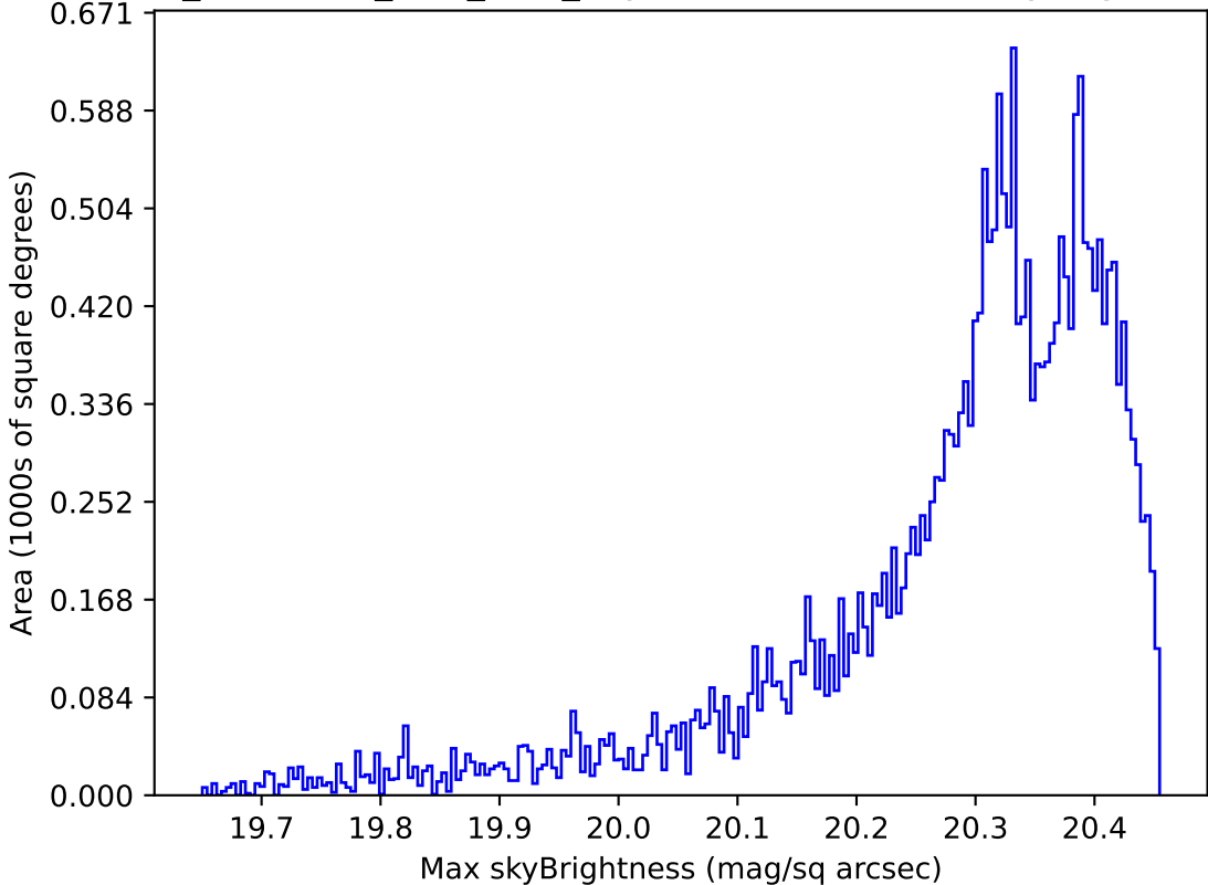
too_combined_s0.5_v3.4_10yrs Yr 1 i band: Max skyBrightness
