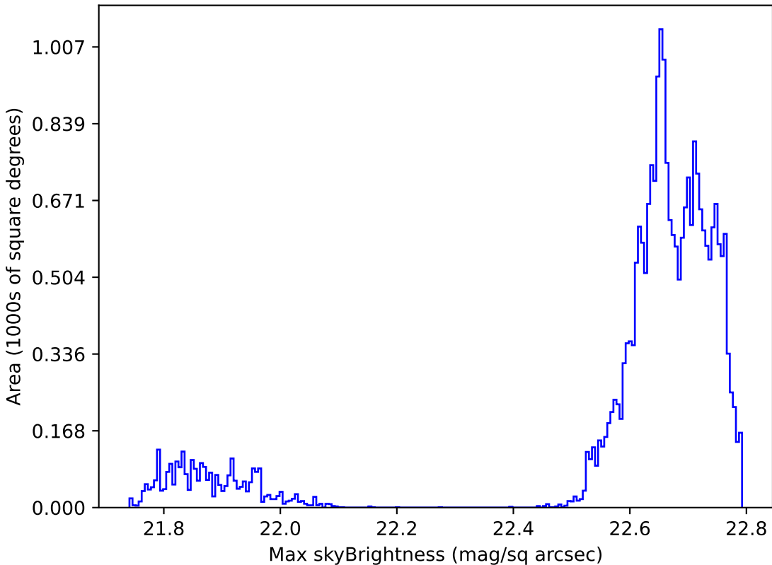
too_combined_s0.5_v3.4_10yrs Yr 1 all bands: Max skyBrightness
