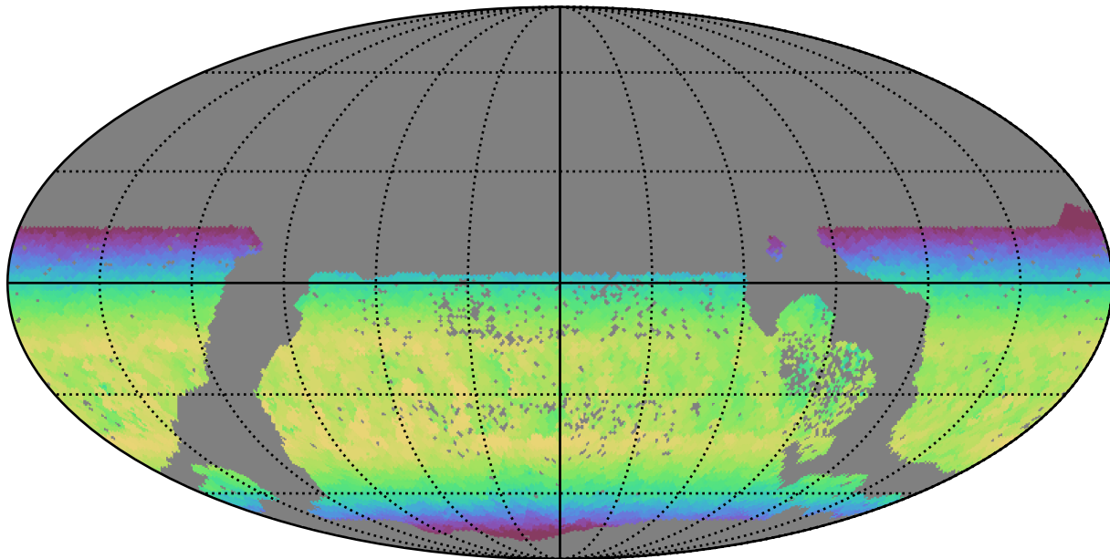
too_combined_s0.5_v3.4_10yrs WFD y band: Max skyBrightness
