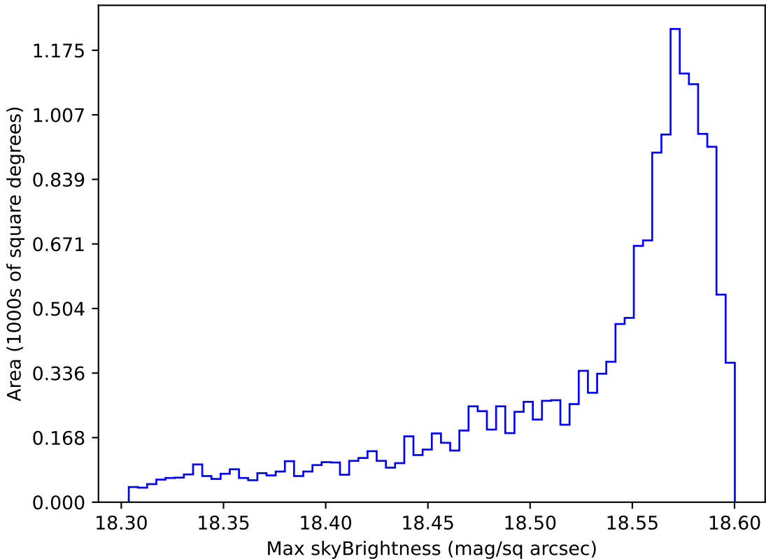
too_combined_s0.5_v3.4_10yrs WFD y band: Max skyBrightness
