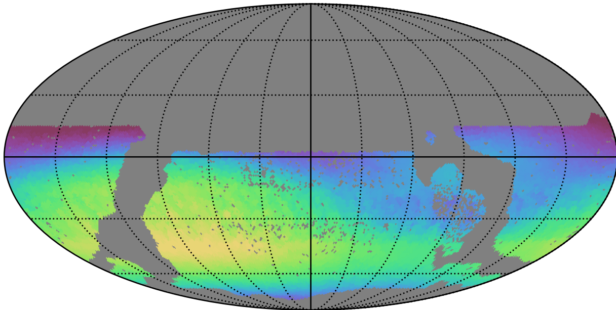
too_combined_s0.5_v3.4_10yrs WFD u band: Max skyBrightness
