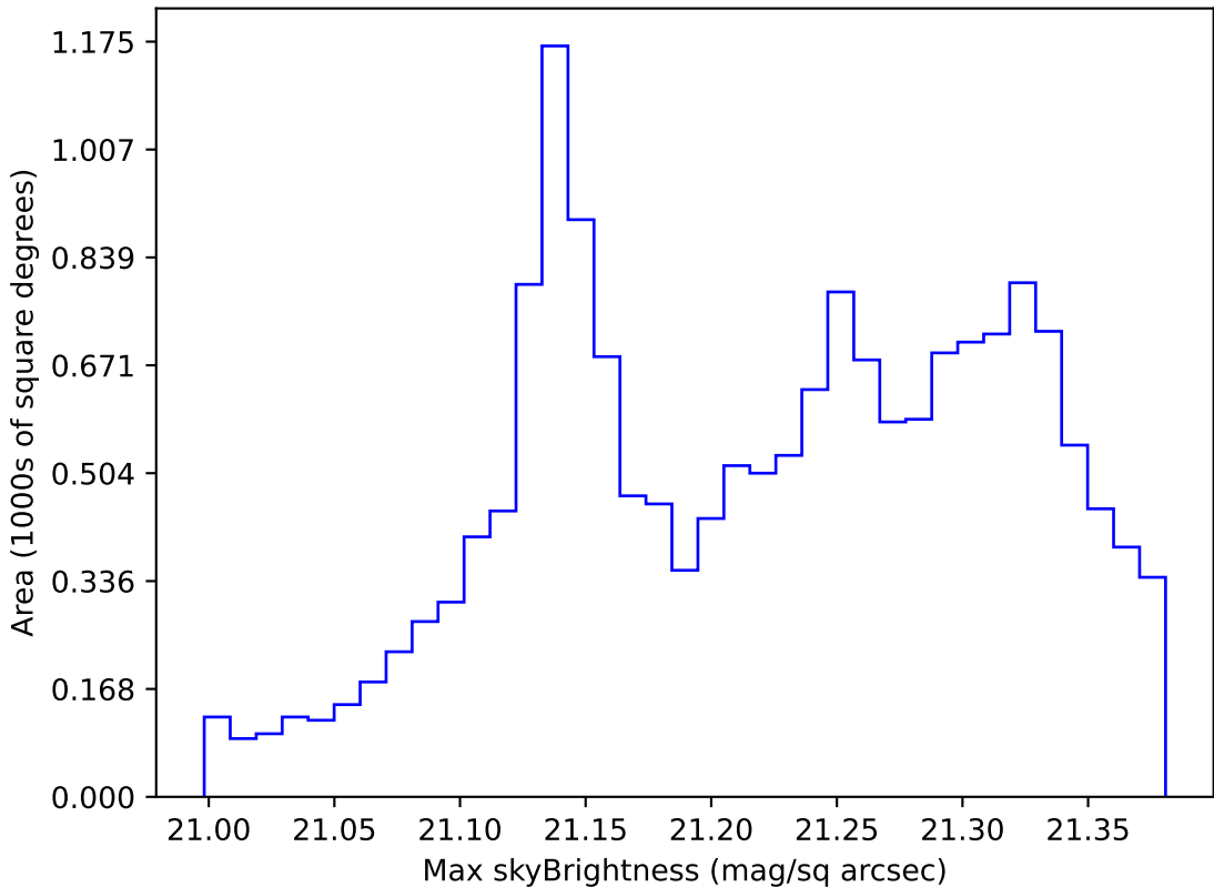
too_combined_s0.5_v3.4_10yrs WFD r band: Max skyBrightness
