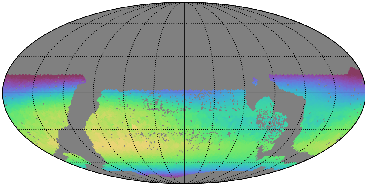
too_combined_s0.5_v3.4_10yrs WFD i band: Max skyBrightness
