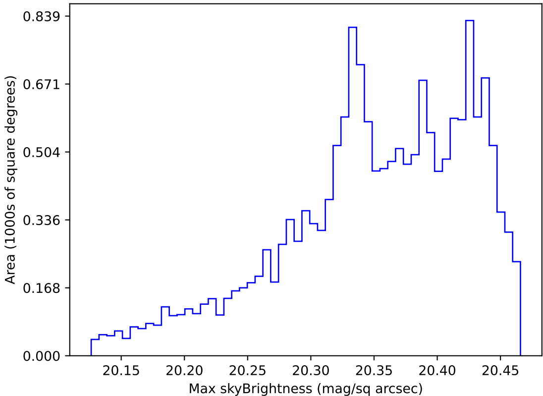
too_combined_s0.5_v3.4_10yrs WFD i band: Max skyBrightness
