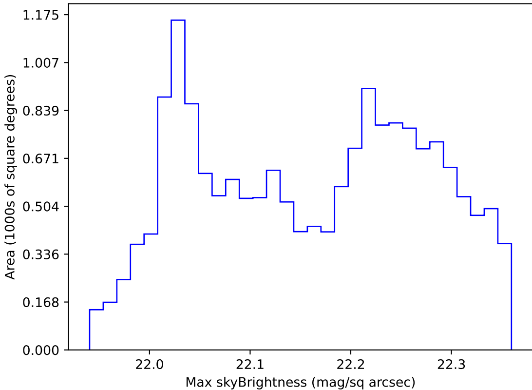
too_combined_s0.5_v3.4_10yrs WFD g band: Max skyBrightness
