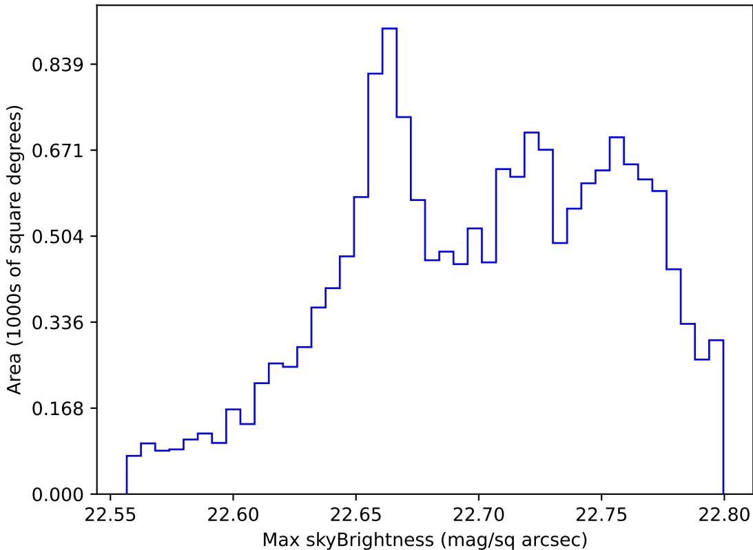
too_combined_s0.5_v3.4_10yrs WFD all bands: Max skyBrightness
