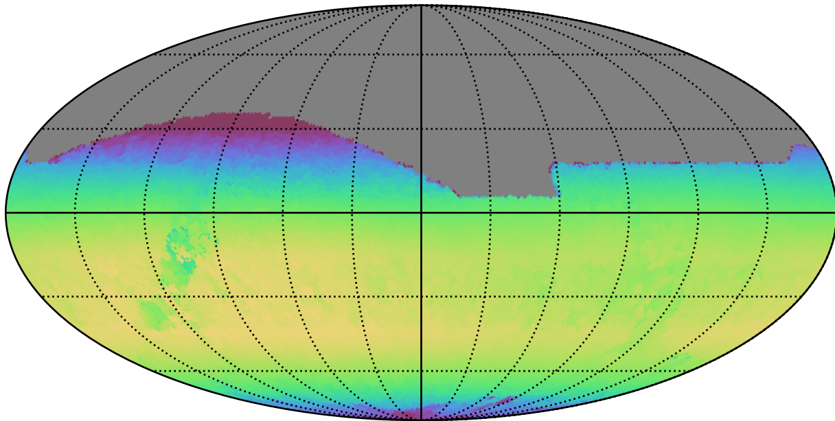
too_combined_s0.5_v3.4_10yrs All sky z band: Max skyBrightness
