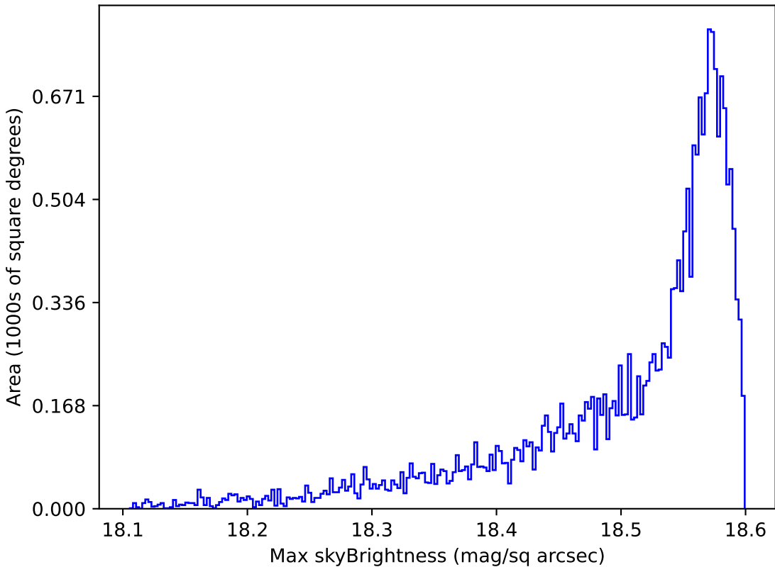
too_combined_s0.5_v3.4_10yrs All sky y band: Max skyBrightness
