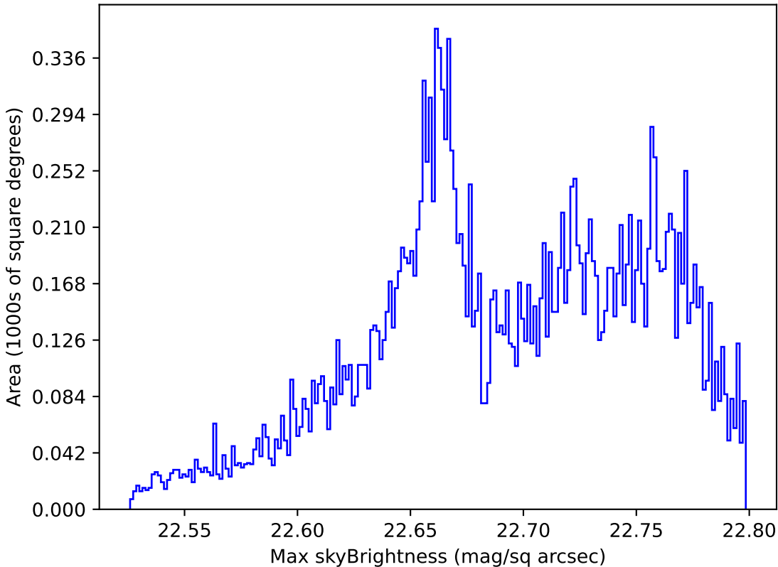
too_combined_s0.5_v3.4_10yrs All sky u band: Max skyBrightness
