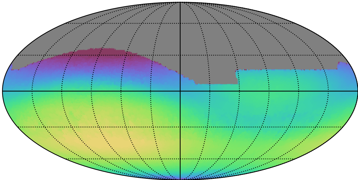
too_combined_s0.5_v3.4_10yrs All sky r band: Max skyBrightness
