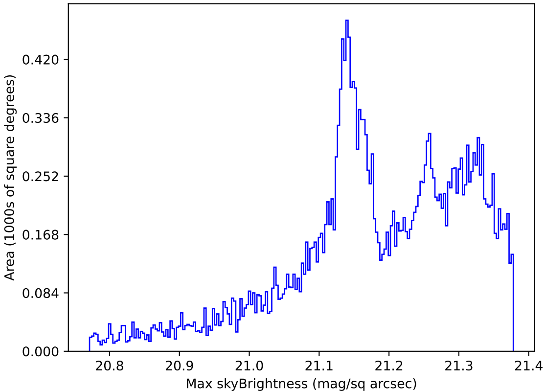
too_combined_s0.5_v3.4_10yrs All sky r band: Max skyBrightness
